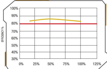
Loading (% of Rated Output Power) — Efficiency %
